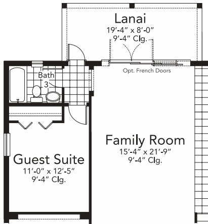
Opt. Guest Suite at Bedroom 5 Ext. Family Room & Ext. Lanai
